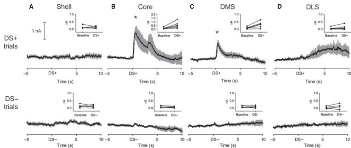
FIG. 5. Discriminative stimuli differentially evoke phasic dopamine signaling across striatal subregions. Average dopamine (black line) \pm SEM (gray vertical bars) to predictive cues in striatal subregions during the discriminative stimulus test. Top – a cue predictive of reward (DS+) selectively evokes phasic dopamine release in the nucleus accumbens core (Core; B) and dorsomedial striatum (DMS; C), but not the nucleus accumbens shell (Shell; A) or dorsolateral striatum (DLS; D). Insets – average dopamine signal for each rat during both Baseline and Cue epochs. Note that in the Core (B), the scale for the ordinate is 2 nA, twice that of the other striatal regions. *P < 0.05 for Baseline vs. DS+ epoch. Bottom – a cue predictive of no reward (DS-) fails to alter phasic dopamine signaling in all striatal subregions. Insets – average dopamine concentration for each rat during both Baseline and Cue epochs.
